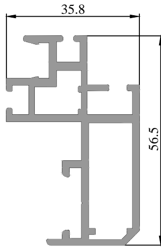
39 1302 00 1.071 kg/m.
