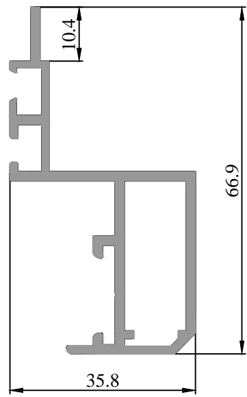
39 1203 00 0.843 kg/m
