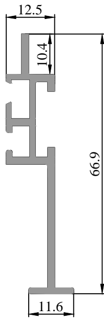
39 1201 00 0.523 kg/m
