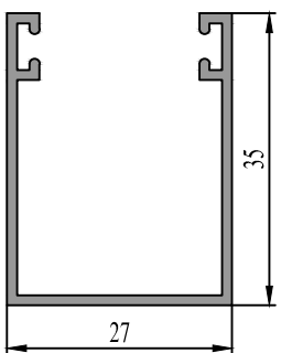
37 0758 12 0.358 kg/m.
