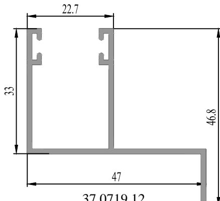
37 0719 12 0.455 kg/m.
