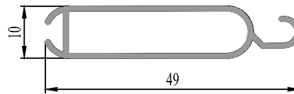
37 0749 00 0.268 kg/m.
