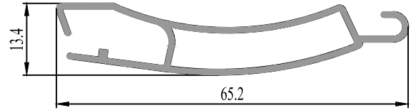
37 0728 10 0.399 kg/m.
