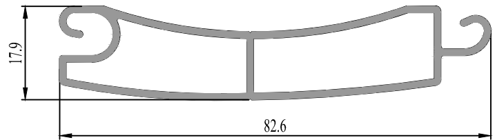
37 0756 12 0.701 kg/m.
