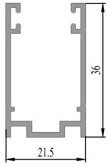
37 0714 12 0.364 kg/m.
