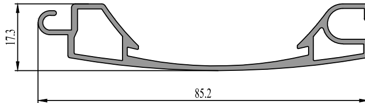
90 5023 00 0.677 kg/m.
