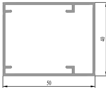
37 0735 12 0.641 kg/m.
