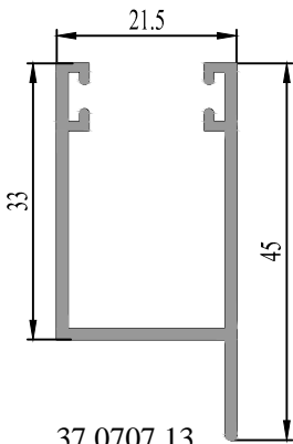
37 0707 13 0.383 kg/m.
